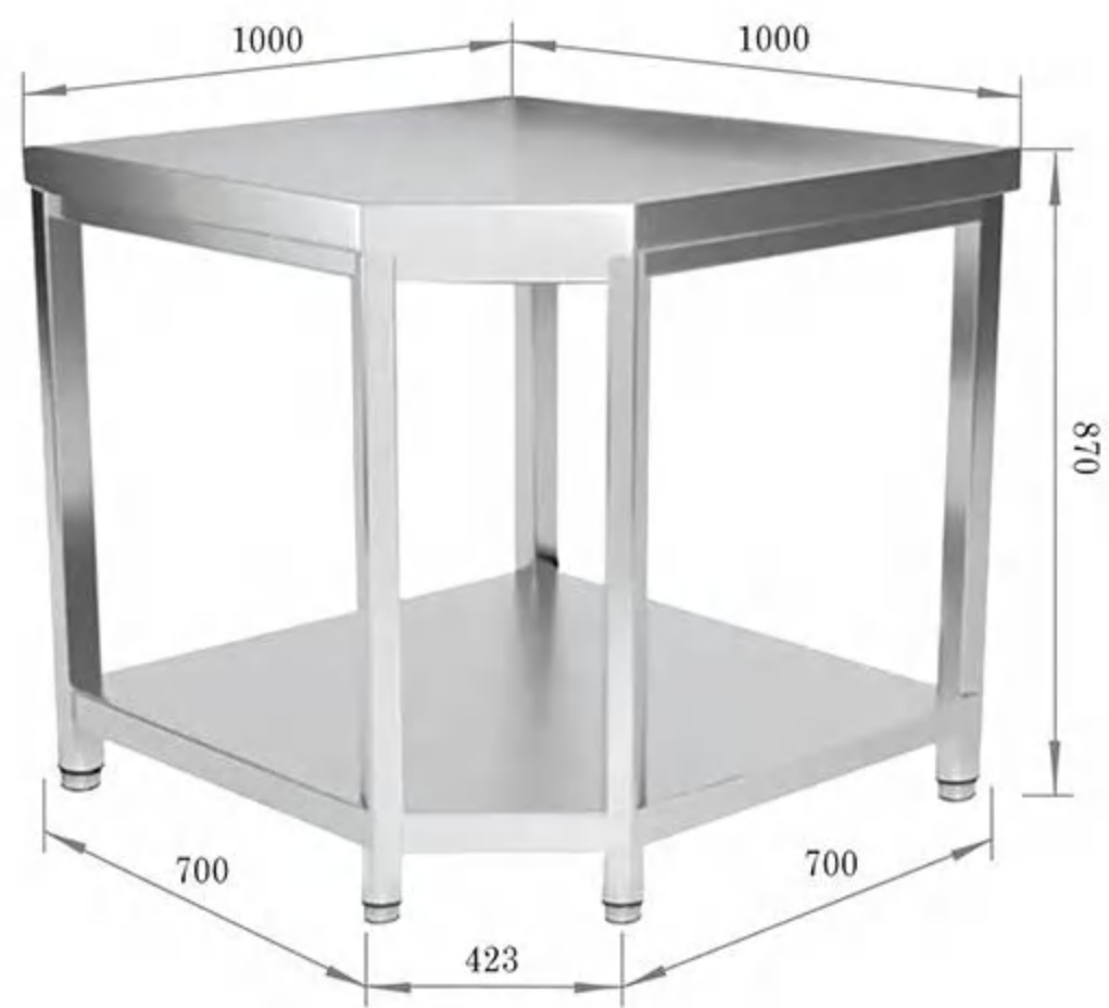
Work table without backsplash
