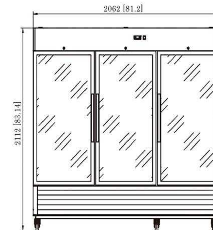
Front view
