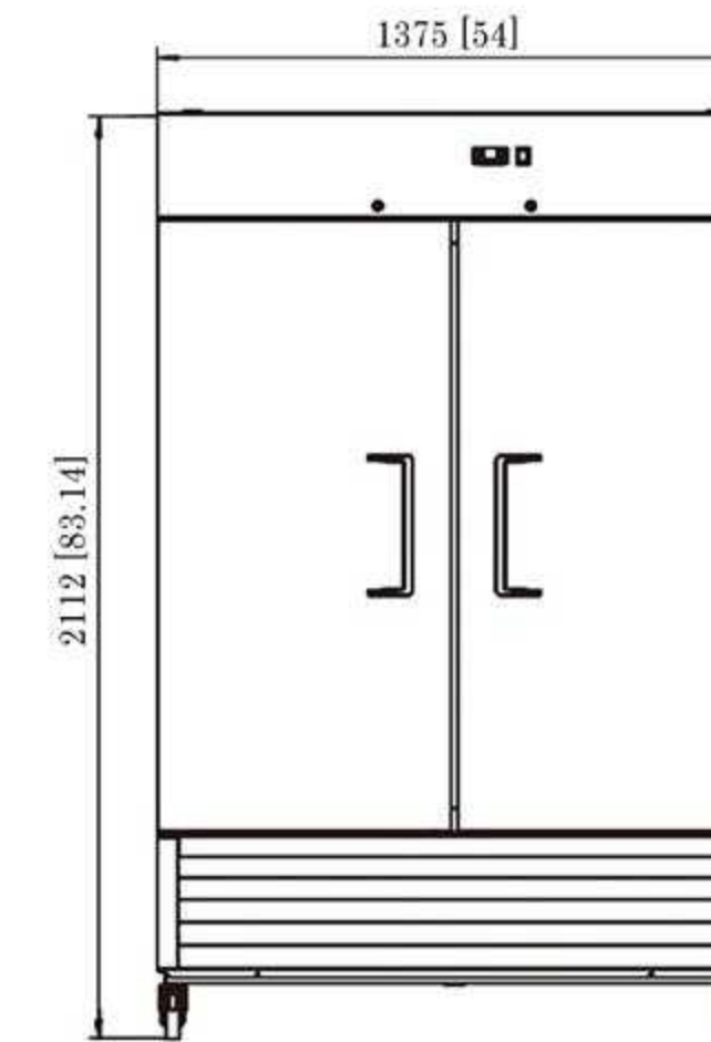
Front view
