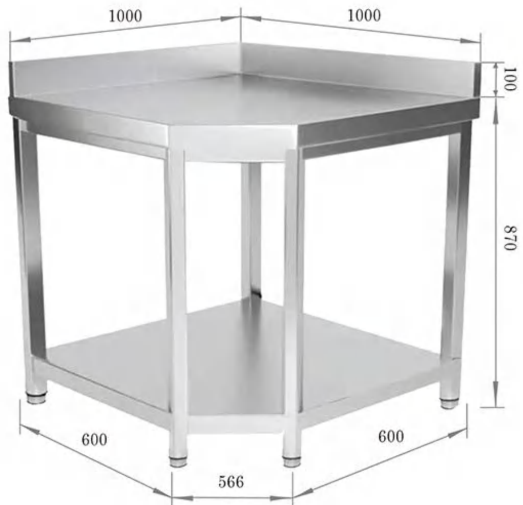
Work table with backsplash
